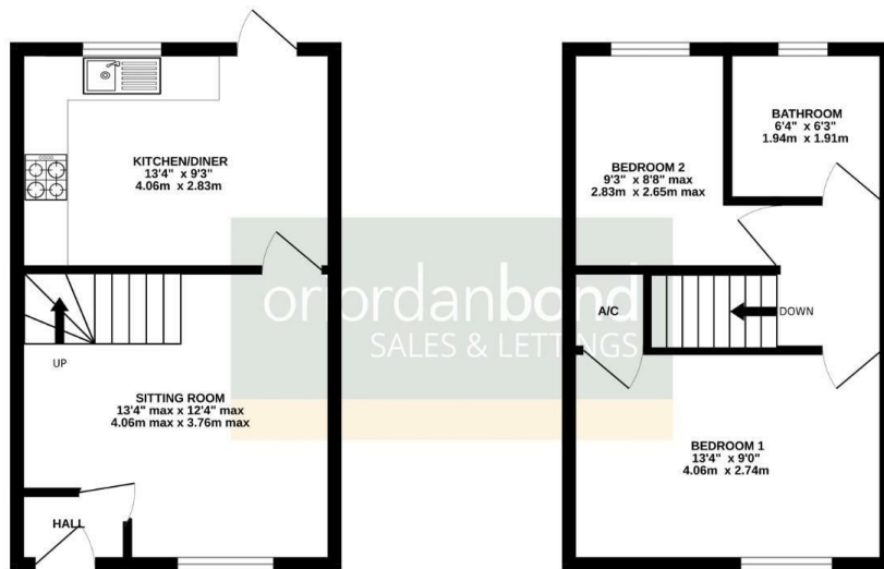
GROUND FLOOR 288 sq.ft. (26.8 sq.m.) approx.
